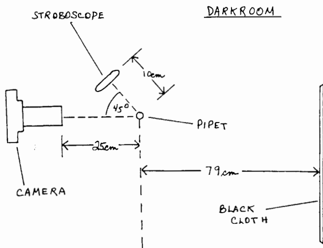
FIG. 5—Photographic equipment in the darkroom.
