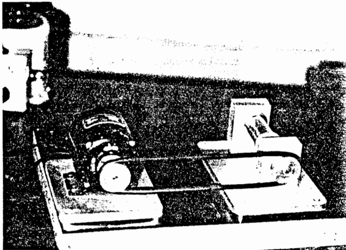
FIG. 2—Drive spool and motor (1/8 hp, 5000 rpm). (1 hp = 746 W).
